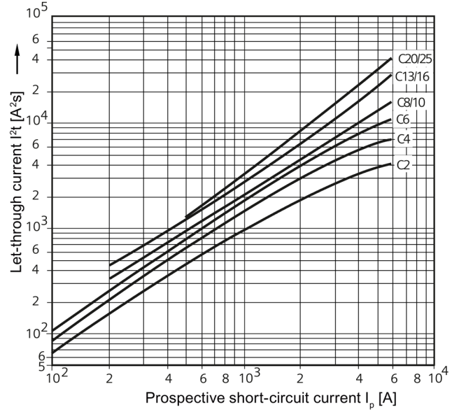
Characteristic C (2 A to 25 A)
