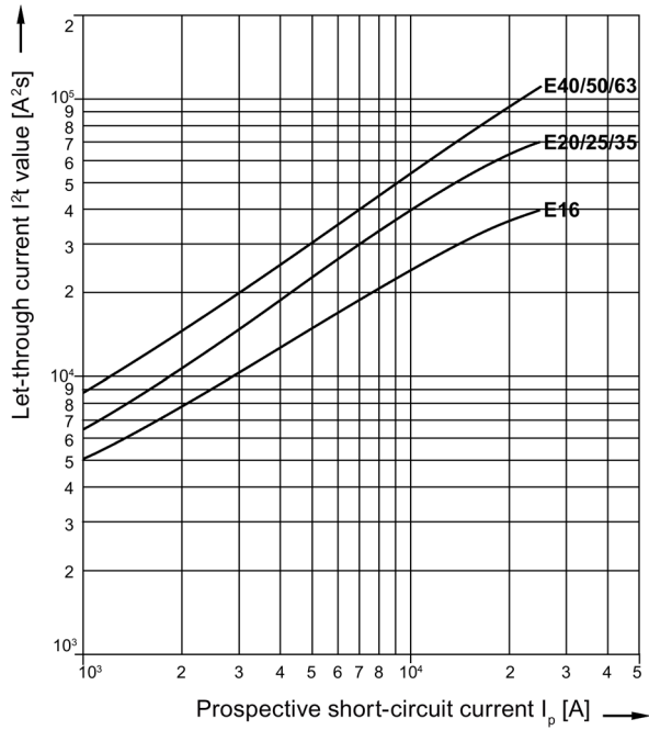
Let-through current 5SP3...-3
