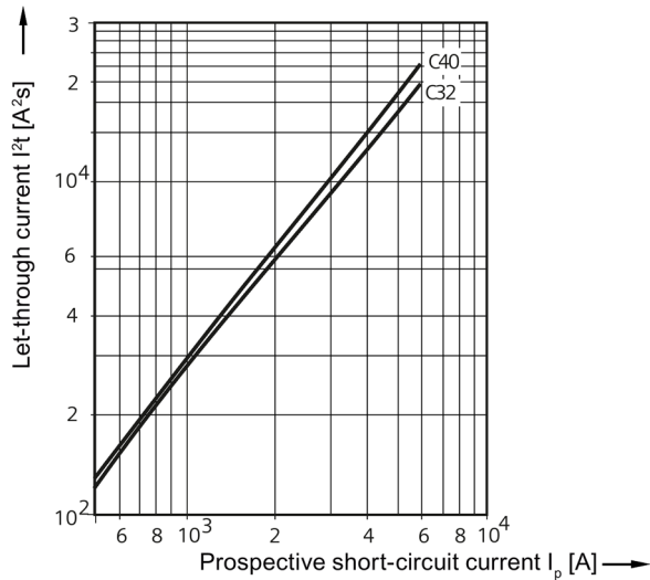
Characteristic C (32 A to 40 A)
