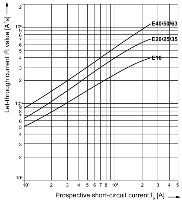
Let-through I^2t values 5SP3...-3
