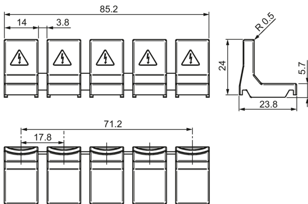
Figure 8-1 5ST3655-0HG
