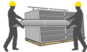
3) Place the stand supporter that is higher or wider than the module in order to avoid hitting and damaging the glass.
