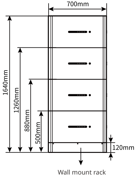
Battery group dimensions (wall-mount installation)
